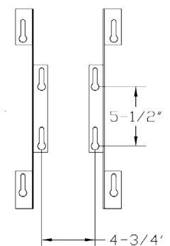
BRACKET MOUNT
