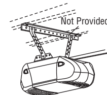
FIGURE 2 Finished Ceiling
