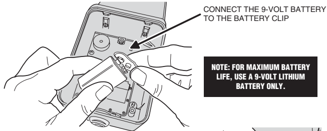
SLIDE THE BATTERY INTO THE BATTERY RETAINING CLAMP
