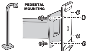
PEDESTAL MOUNTING MOUNT BACKPLATE WITH SECURITY BOLTS AND LOCKNUTS
