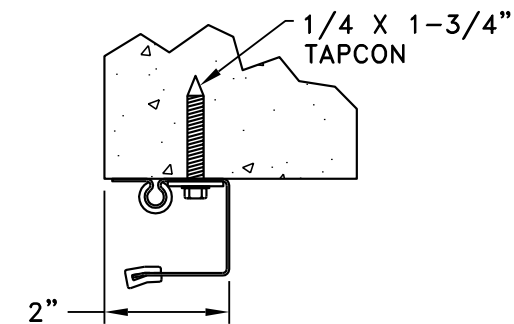
MASONRY JAMB DETAIL
