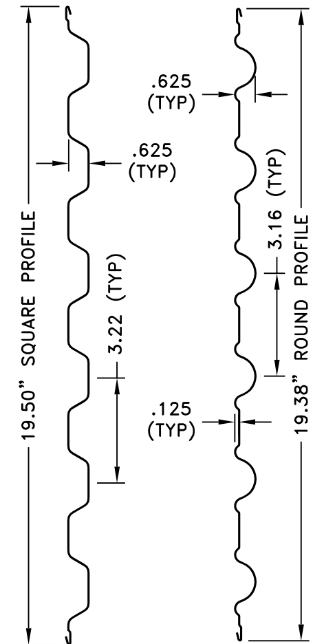
CURTAIN DETAIL (26GA PAINTED GALV. STEEL)
