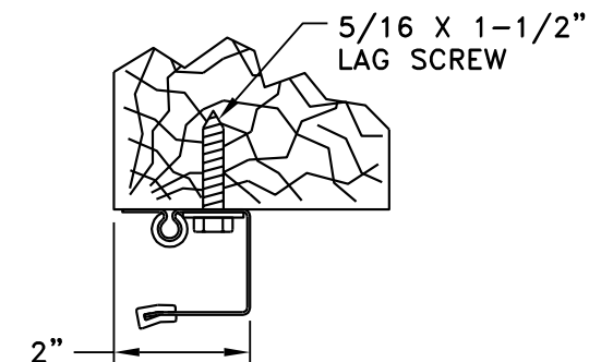
WOOD JAMB DETAIL
