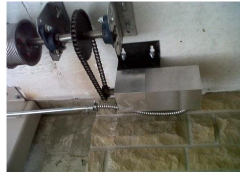
Installed GearMotor with GDI's mounting bracket
