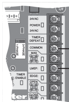
Wiring Connections (Logic 4 board shown)
