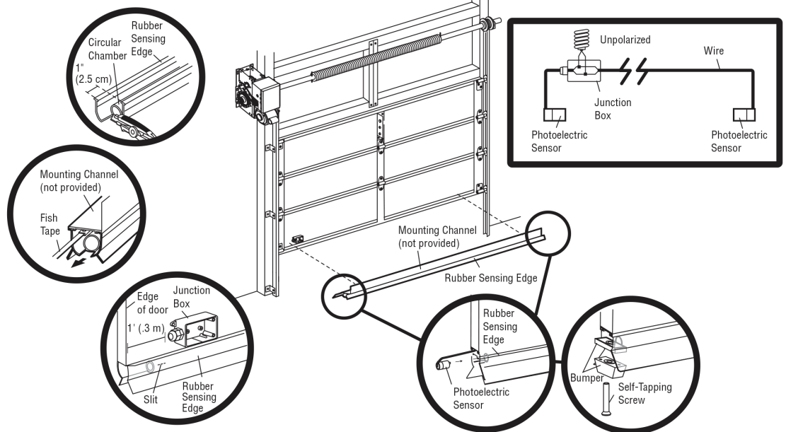
Door with Edge installation shown (See installation manual for complete installation instructions).
