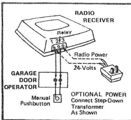
Figure 2. Two-terminal operator: Receiver powered by a step-down transformer.
