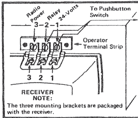
Figure 1. For three-terminal operators: Receiver is shown electro-mechanically attached to operator with terminal mounting brackets.
