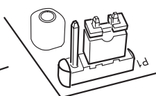
SHUNT SET FOR "STANLEY" OPERATION
