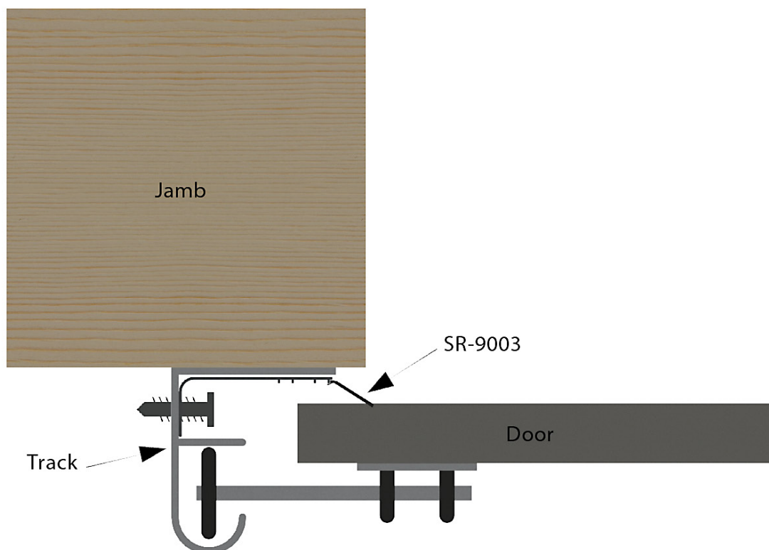
Assembled Profile
