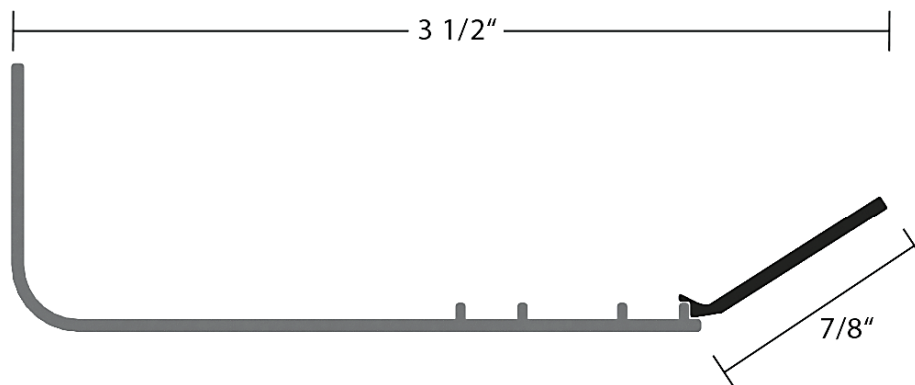
Assembled Profile
