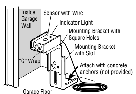
Figure 5 Alternate Floor Mount
