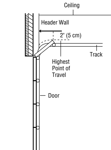
SECTIONAL DOOR WITH CURVED TRACK
