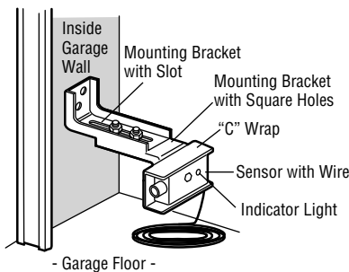
Figure 4 Alternate Wall Mount
