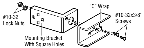
Figure 2 Garage WALL Installation
