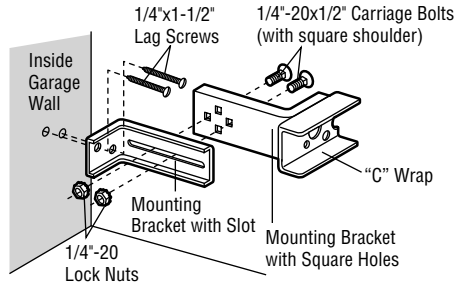
Figure 2 Garage WALL Installation
