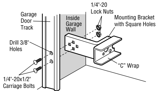
Figure 3 Garage DOOR Track Installation
