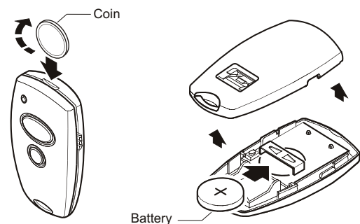
Figure 2. Battery Compartment
